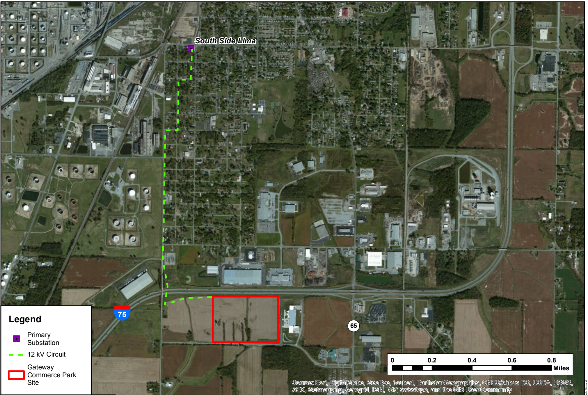
Coordinate System: NAD 1983 StatePlane Ohio North FIPS 3401 Feet Exhibit 4.1.2: Substation-Overhead Electric Powe Lines
